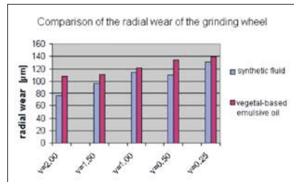
Figure 4. Comparison of the radial wear of the grinding wheel.
