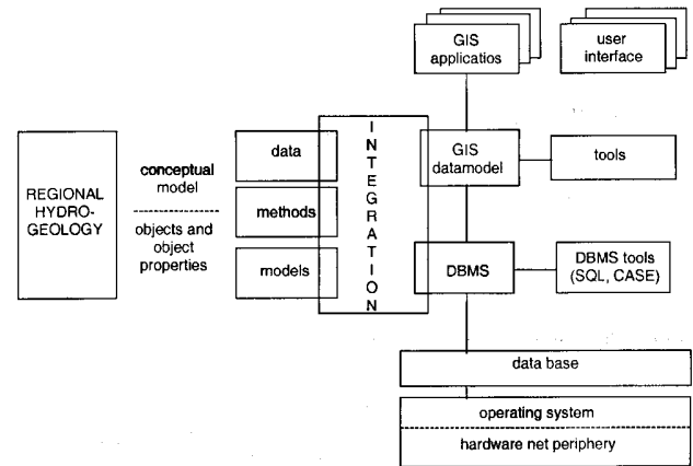
Figure 5. Managing hydrogeologic data in a GIS (modified after Schilcher et al. , 1996).
