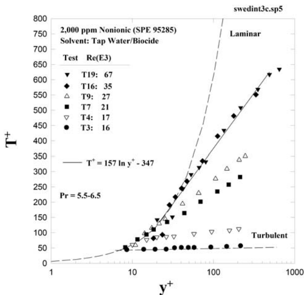
FIGURE 9. Temperature profiles for a 2000 ppm non-ionic surfactant solution diluted in tap water. In this case, the increase in the DR (and HTR ) level is reflected as an increase in the slope of the buffer layer, even at low levels of reduction. These are the Fan-Type profiles.
