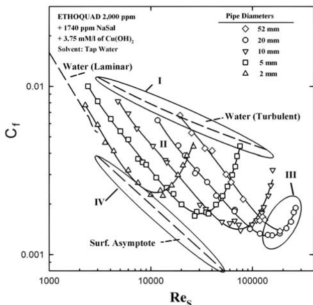
FIGURE 1. Friction coefficients for five pipe diameters (52, 20, 10, 5 and 2 mm) as a function of solvent Reynolds number for an Ethoquad T13/27 solution: 2,000 ppm, plus 1,740 ppm of NaSal, plus 3.75 mM/l of \text{Cu}(\text{OH})_2 . The maximum drag reduction asymptote (MDRA) for surfactants proposed by Zakin et al. [21] is shown as a reference. Temp = 20°C. The regions labeled with numbers I, II, III, and IV represent the vicinity of the onset, intermediate, super-critical, and asymptotic regions. Note that regions I and IV always correspond to the vicinity of the turbulent Newtonian friction coefficient, and the MDRA, respectively. Regions II and III may vary for different C_f curves. Region III is only marked for the 20 mm diameter pipe data.
