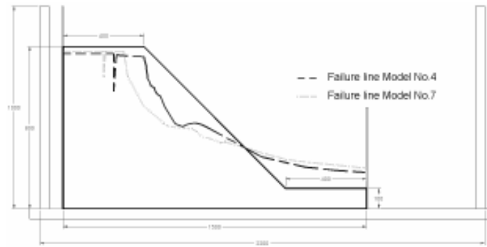
Figure 9. Final contour failure models No. 4 and No. 7 Figura 9. Contorno final de falla Modelos No. 4 y No. 7
