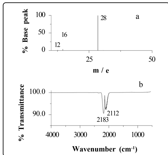
Figure 3. Mass spectrum (a) and infrared spectrum (b) of carbon monoxide formed from \gamma -irradiated Lexan.
